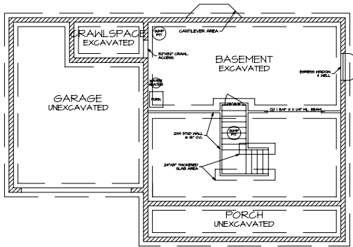
FOUNDATION PLAN A-3 SCALE: 1/4"=1'-0"
