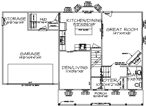
FIRST FLOOR PLAN A-4 SCALE: 1/4"=1'-0"
